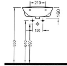
TEK PARÇA LAVABO BATARYA DELİKLİ TPAA02701V00W5000 450x350 mm
