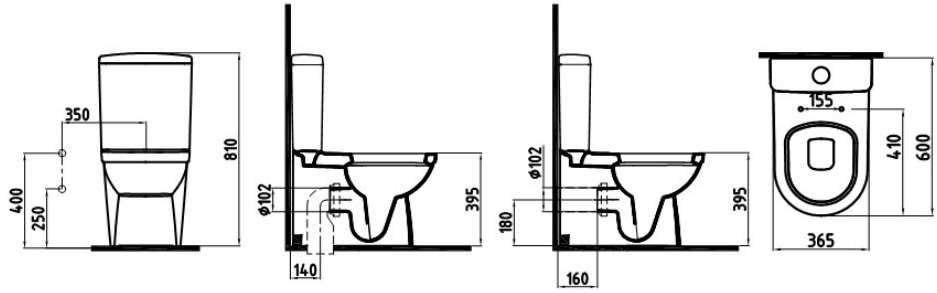
DUVARA SIFIR KLOZET ORKD06001VS1W5S20 600x365 mm
