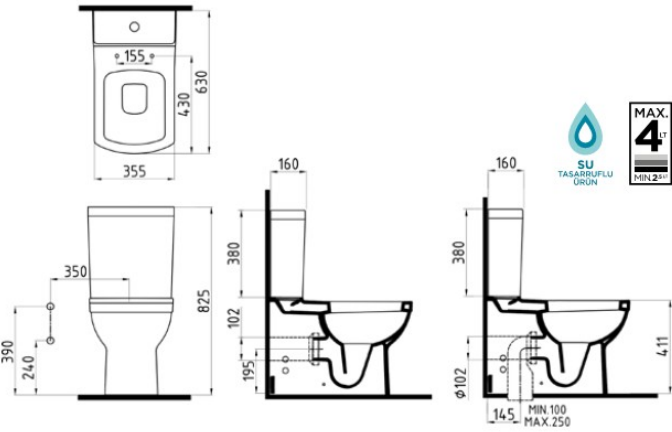
DUVARA SIFIR KLOZET DRKD063B1VS1W5SZ0 630x355 mm
