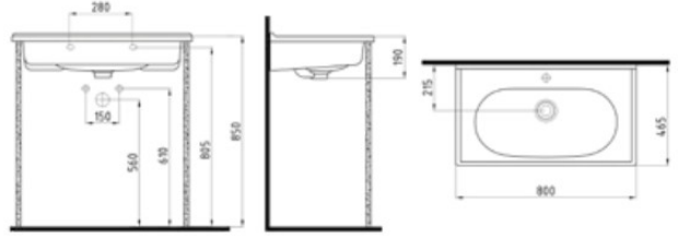
KONSOLLU LAVABO BATARYA DELİKLİ / TAŞMA DELİKLİ FELK080B1FD1W5000 800x465 mm
