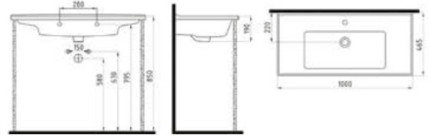
KONSOLLU LAVABO BATARYA DELİKLİ TAŞMA DELİKLİ NPLK10001FD1W5000 1005x470 mm
