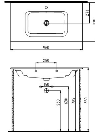
KONSOLLU LAVABO BATARYA DELİKLİ / TAŞMA DELİKLİ CALK09601FD1W5000 960x510mm
