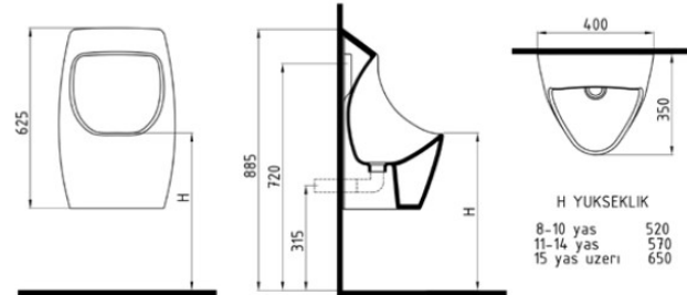
HARMONY SUSUZ PİSUAR 62cm HRPW06201VSSW5000
