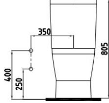
DUVARA SIFIR KLOZET NPKD06301VS1W5SZ0 630x355 mm
