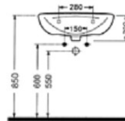
BEDENSEL ENGELLİLER İÇİN LAVABO TPLE06001VD1W3000 600x510 mm
