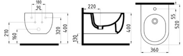
ASMA BİDE MDBA05201VD1W5000 520x360 mm
