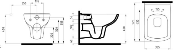
GOYA ASMA KLOZET NO-RIM GYKA052H2VP1W5000 525x355mm
