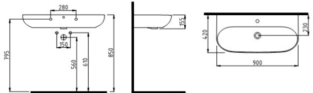
DUVAR MONTAJLI LAVABO BATARYA DELİKLİ / TAŞMA DELİKLİ MDLS09001FD1W5000 900x420 mm
