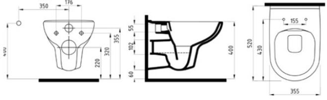
LEO ASMA KLOZET NO-RİM LEKA052H2VP1W5000 520x355 mm
