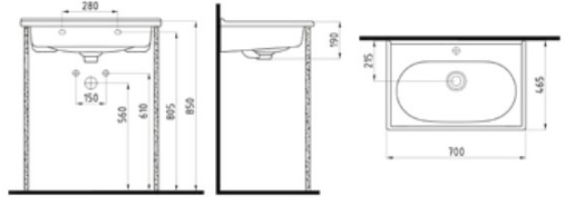
KONSOLLU LAVABO BATARYA DELİKLİ / TAŞMA DELİKLİ FELK070B1FD1W5000 700x465 mm
