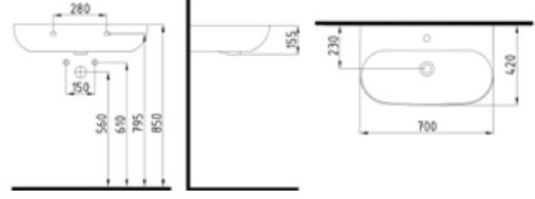
DUVAR MONTAJLI LAVA- BO BATARYA DELİKLİ / TAŞMA DELİKLİ MDLS07001FD1W5000 700x420 mm
