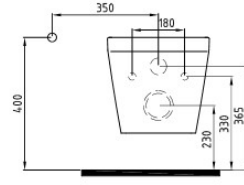
ASMA KLOZET 52 cm TAHARET BORULU NPKA052AMVP1W5000 520x350 mm
