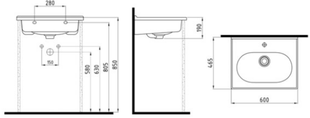
KONSOLLU LAVABO BATARYA DELİKLİ / TAŞMA DELİKLİ FELK060B1FD1W5000 600x465 mm
