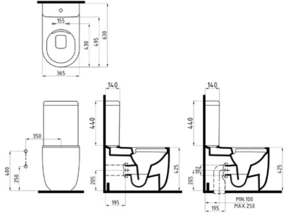
DUVARA SIFIR KLOZET MDKD063N1VS1W5SZ0 630x365 mm
