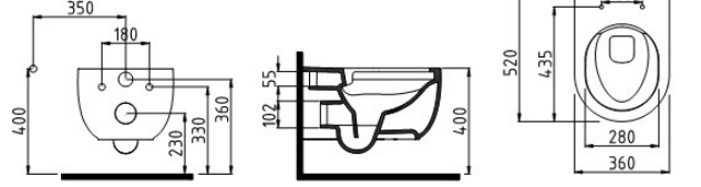
ASMA KLOZET NO-RİM MDKA052N1VP1W5000 520x360 mm Beyaz 1.003 TL
