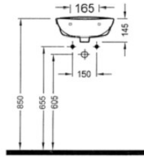
TEK PARÇA LAVABO BATARYA DELİKSİZ TPLS03601VD0W5000
