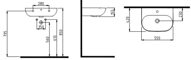
DUVAR MONTAJLI LAVABO BATARYA DELİKLİ / TAŞMA DELİKLİ MDLS05501FD1W5000 550x420 mm
