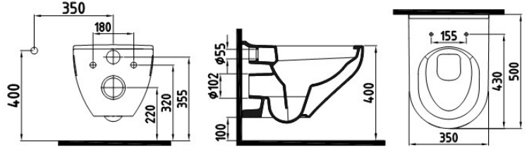
NO-RIM ASMA KLOZET IOKA050N2VP1W5000 500x350 mm
