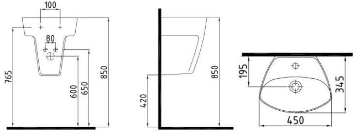
MONOBLOK LAVABO BATARYA DELİKLİ / TAŞMA DELİKLİ MNLM04501FD1W5000 450x350 mm
