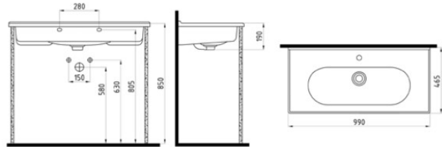
KONSOLLU LAVABO BATARYA DELİKLİ / TAŞMA DELİKLİ FELK100B1FD1W5000 1000x465 mm
