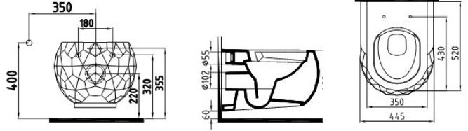
NO-RIM ASMA KLOZET PNKA052N1VP1W3000 520x350 mm
