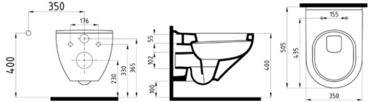
ASMA KLOZET IOKA050AMVP1W5000 500x350 mm
