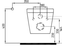
N1 NO-RIM ASMA KLOZET NPKA052N1VP1W5000 520x350 mm
