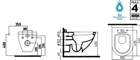
ASMA KLOZET 52 cm TAHARET BORULU HRKA052AMVP1W5000 520x350 mm
