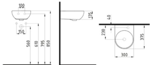
DUVAR MONTAJLI LAVABO BATARYA DELİKLİ / TAŞMA DELİKLİ MDLS03001FD1W5000
