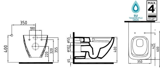
NO-RIM ASMA KLOZET KRKA060N1VP1W3000 600x350mm
