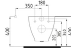
H1- NO-RIM ASMA KLOZET HRKA054HVP1W5000 540x350 mm
