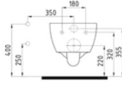
N3- NO-RIM ASMA KLOZET HRKA052N3VP1W3000 530x350 mm
